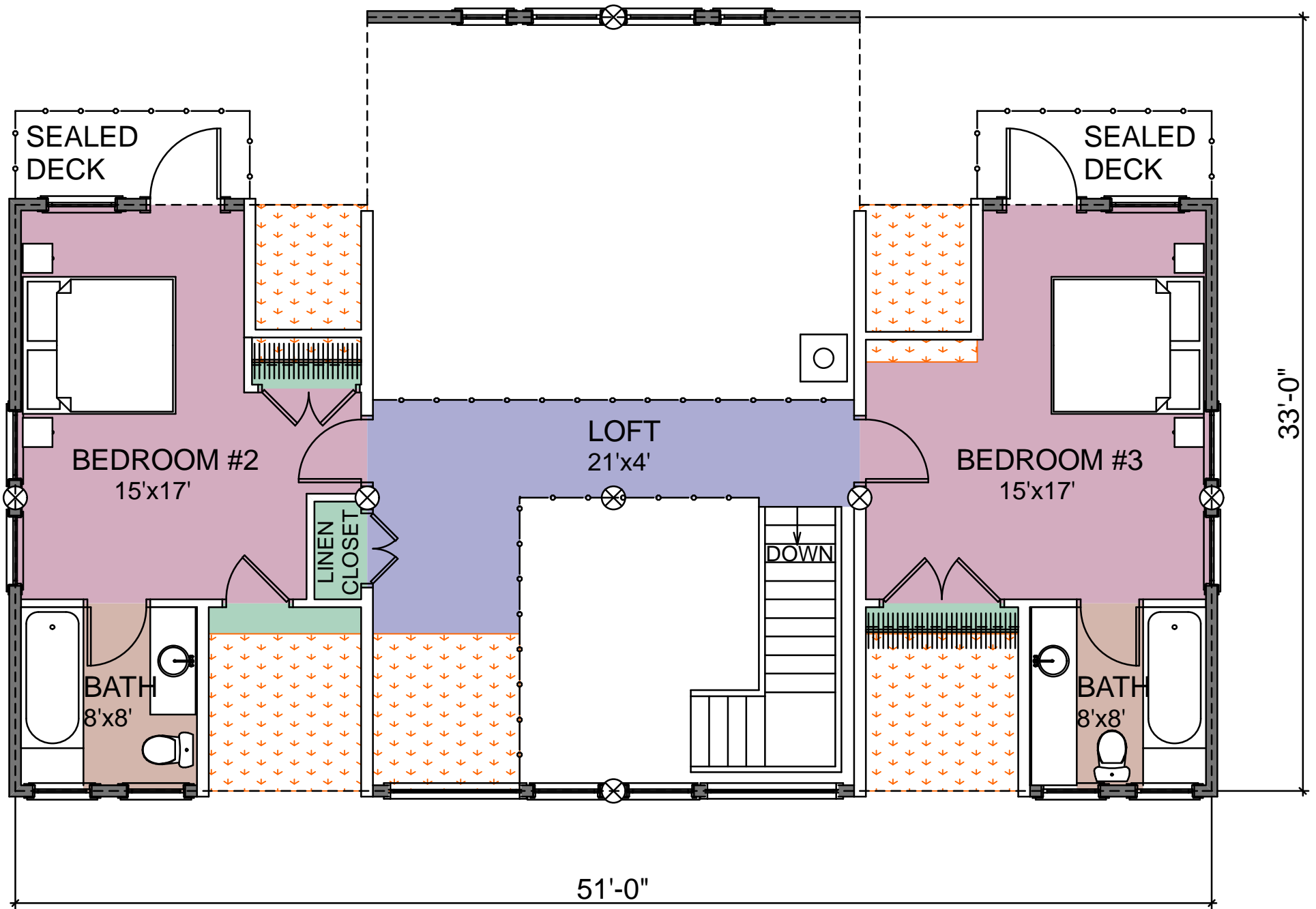
SECOND FLOOR PLAN AREA: 784 SQ. FT.
