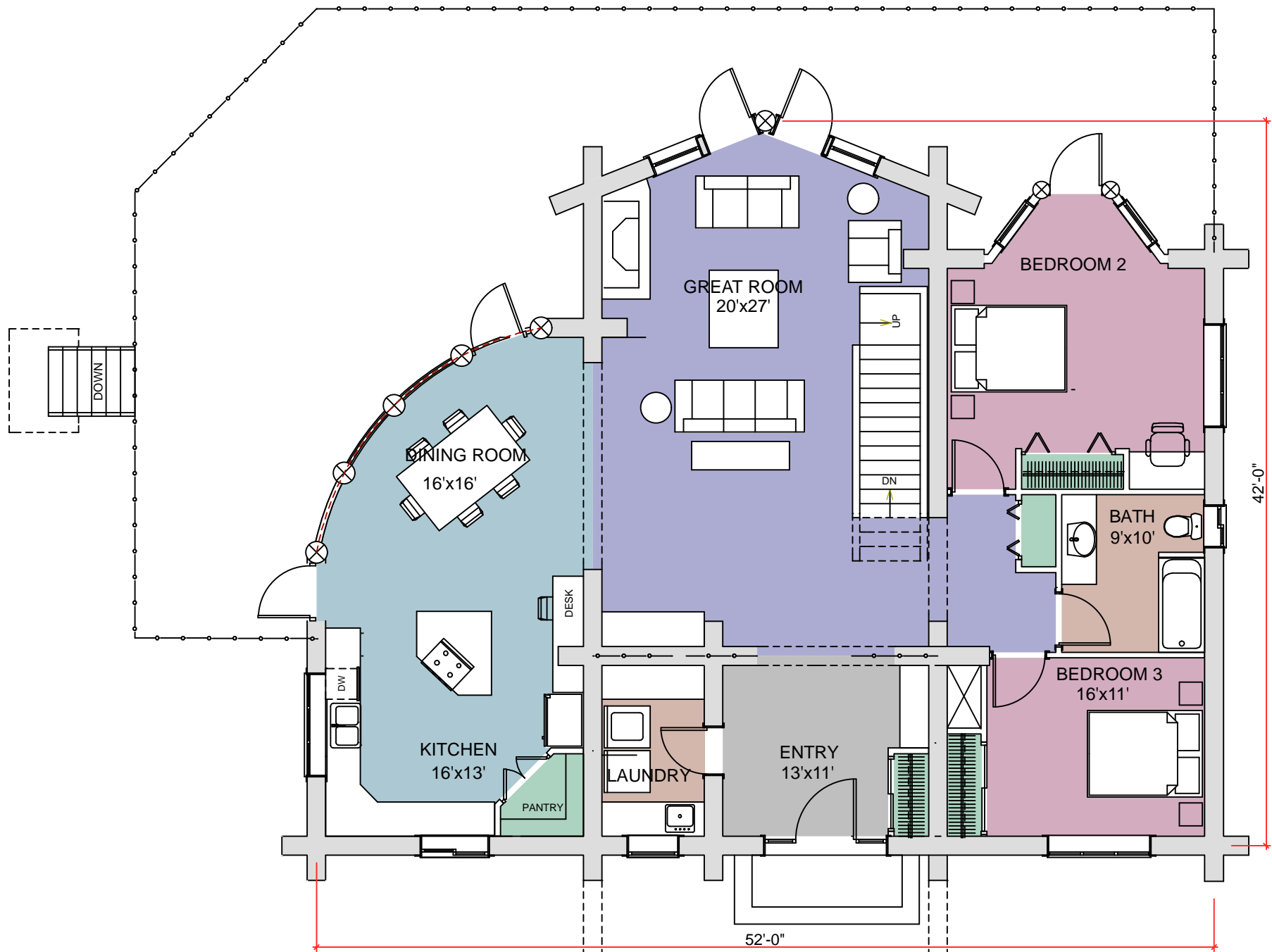
FIRST FLOOR PLAN AREA : 1,877 SQ.
